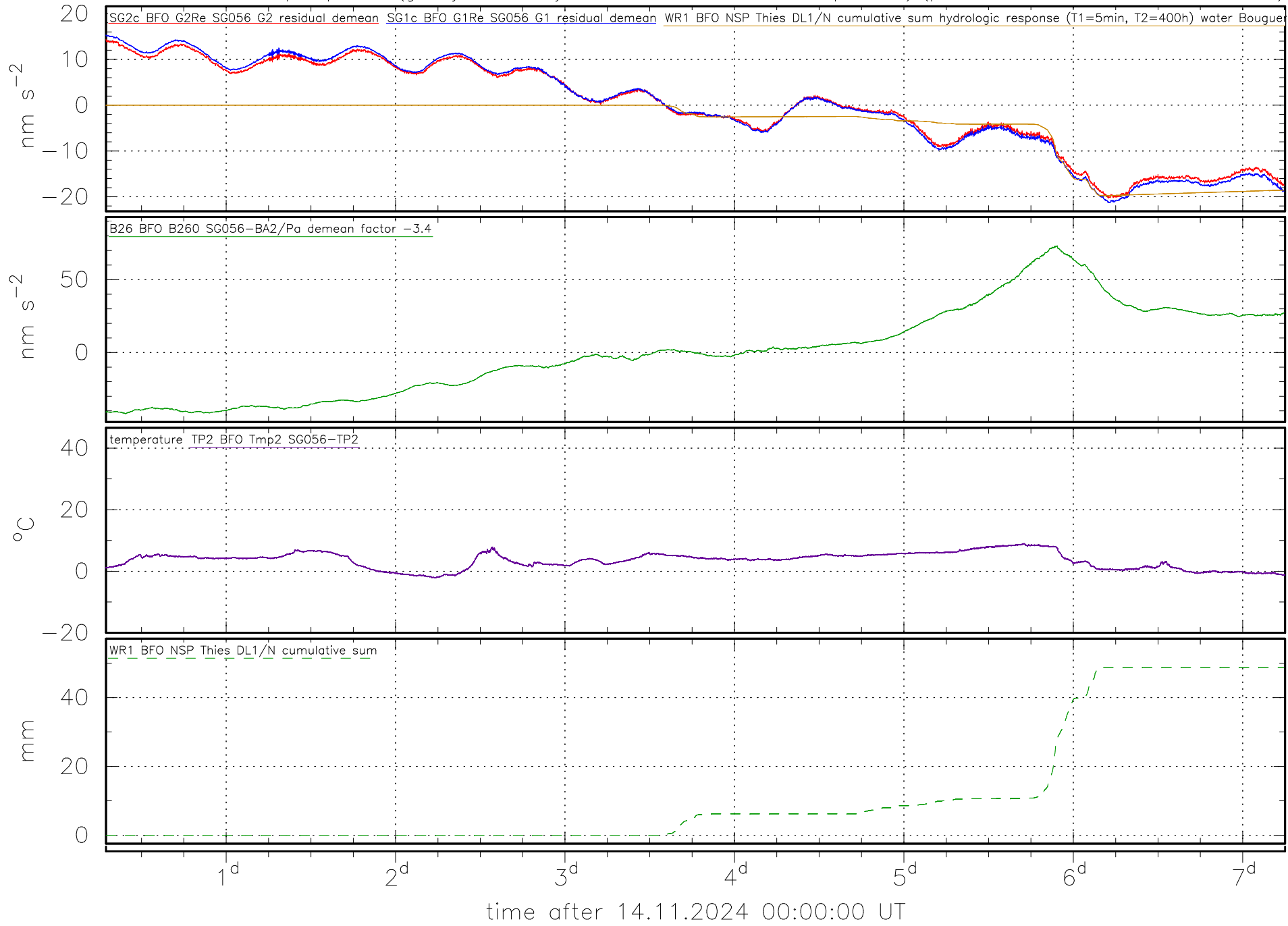
SG056 residuals vs. precipitation (gravity reduced by: drift, tidal model, scaled air-pressure) (plot created at 21.11.2024 06:58:46 UT)
